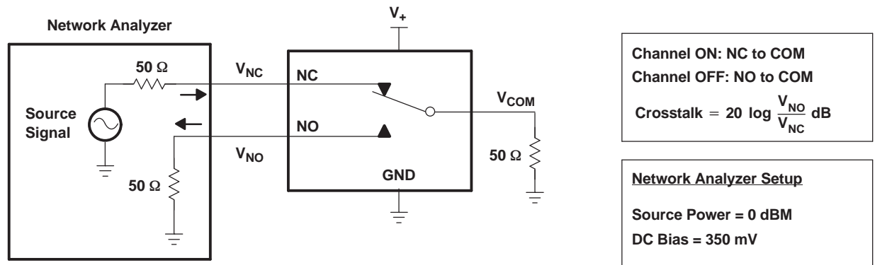
Figure 21. Crosstalk ( X_{TALK} )
