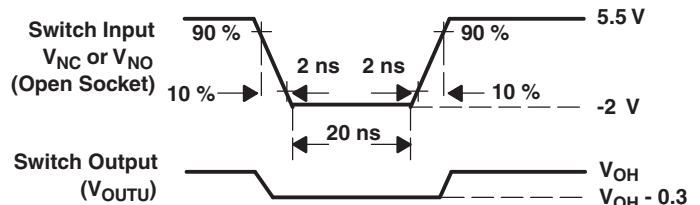
Switch Input and Output for Undershoot Test
